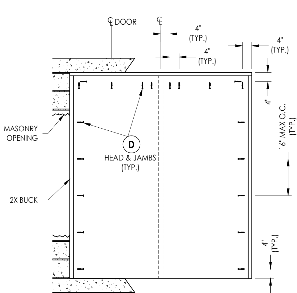
BUCK ANCHORING
